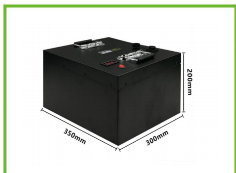
72V40AH Lithium battery pack
